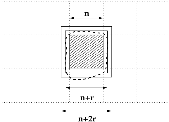
Figure 5: A good square. There is only one component of discs (represented by the dashed line) that intersects both B_{n+2r} and B_{n+r} . This component must reach to within 2\epsilon of all edges of B_{n+r} , and will therefore intersect a component of an adjacent good square.
