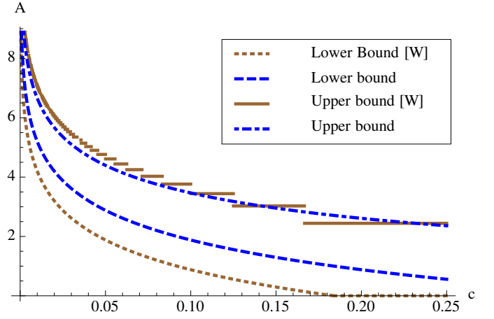
Figure 2. Bounds on \hat{A}(D) + \lg n for D = cn^2 + O(n) where the error terms are ignored. The bounds denoted by [W] are those from [17].
